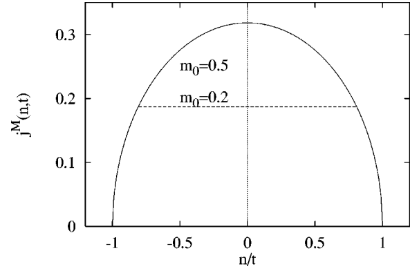
FIG. 2. Scaling functions for the magnetization-current for initial conditions m_0=0.5 and m_0=0.2 as given by Eq. (15).
